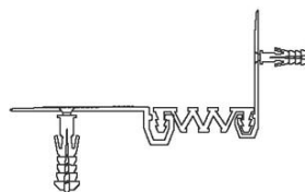
AR262-050 KÖŞE DETAYI AR262-050 CORNER DETAIL
